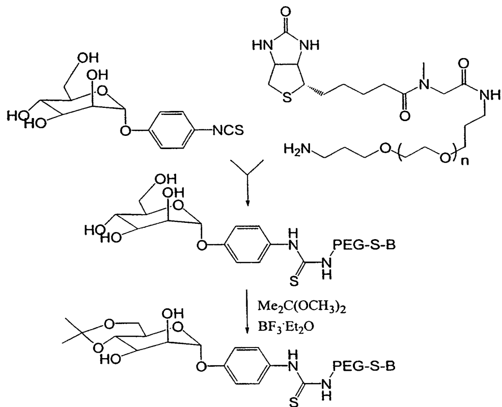
Scheme 11
